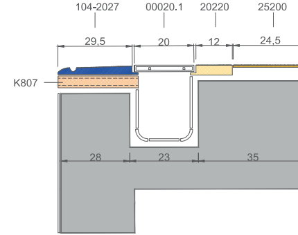
Tünel Sistem Detay-1 / Tunnel System Detail-1
