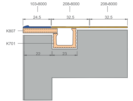
Tünel Sistem Detay-2 / Tunnel System Detail-2
